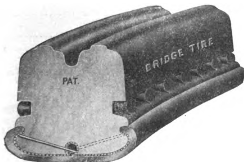
SECTION SWINEHART TWIN TREAD TIRE.
